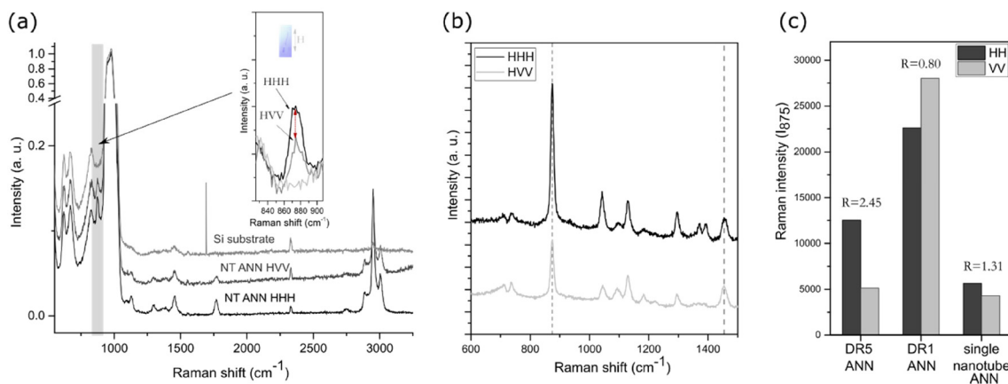
Fig. 4 Polarized Raman spectra of (a) extracted annealed nanotubes in pore length direction (HHH) and perpendicular (HV) for orientation assessment with magnification of 875\text{ cm}^{-1} peak (b) and drawn film in drawing direction (HHH) and perpendicular (VV). (c) Comparison of Raman intensities for horizontal and perpendicular values of 875\text{ cm}^{-1} peak for annealed drawn film (DR5 ANN), non-oriented film (DR1 ANN) and single nanotube, with calculated orientation ratio ( R ) as HHH normalized to VVV values.
