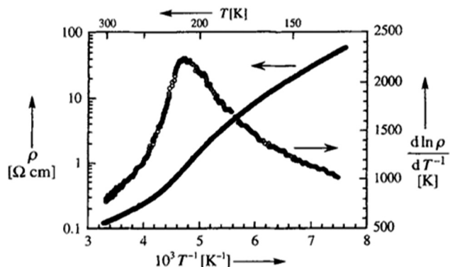
Fig. 4 Electrical resistivity \rho of (DT-TTF) 2 [Au(mnt) 2 ] ( 1 ) as a function of the reciprocal temperature (left) and its first derivative, d \ln \rho / dT^{-1} (right). Reproduced with permission from ref. 27. Copyright 1997 Wiley-VCH.
