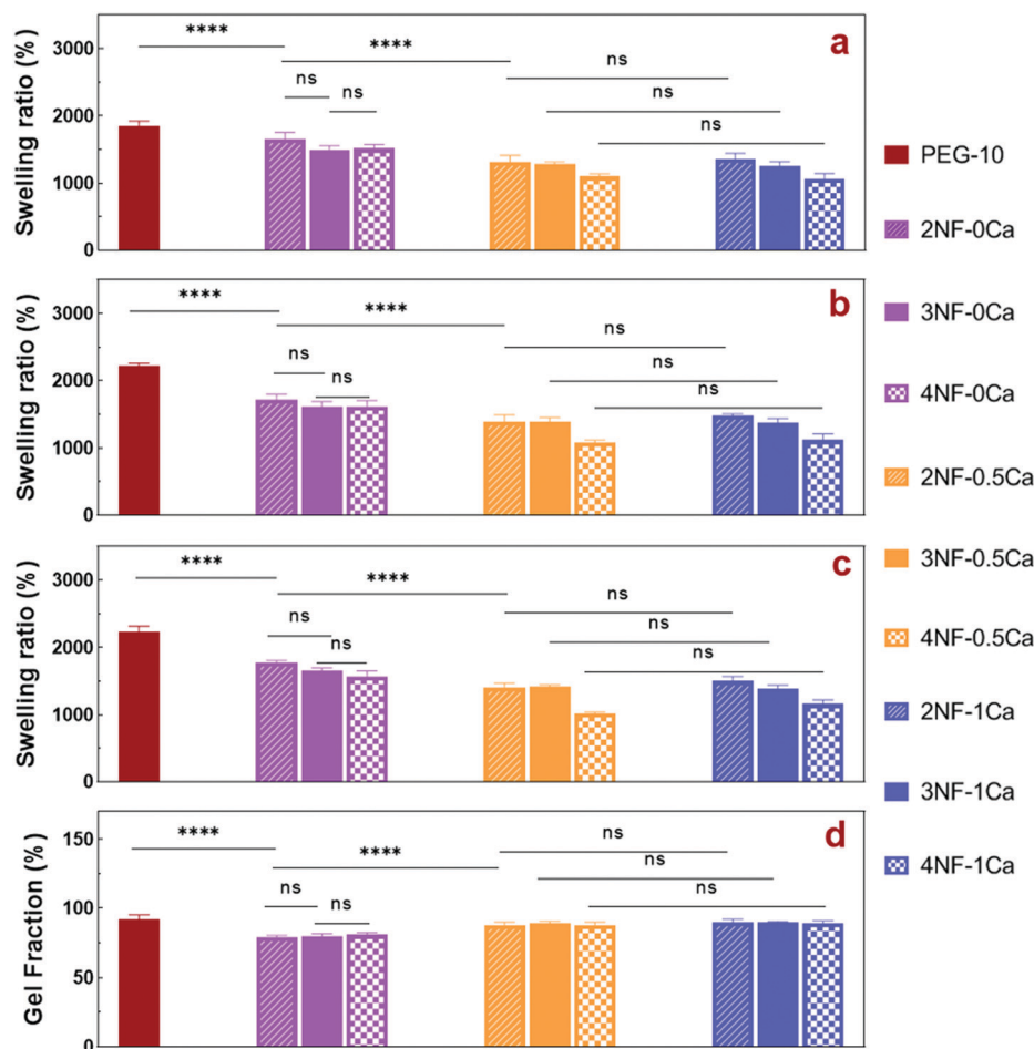
Fig. 5 Water uptake of different PEG-CNF hydrogel inks. Equilibrium mass swelling ratios of PEG-CNF hydrogels formed with various contents of CNFs or Ca 2+ ( n = 5 , mean \pm SD) after (a) 2 h, (b) 9 h, and (c) 24 h incubation in PBS. (d) Gel fractions of PEG-CNF hydrogels after 24 h incubation in water ( p < 0.001 , one-way ANOVA, Tukey's post-test).
