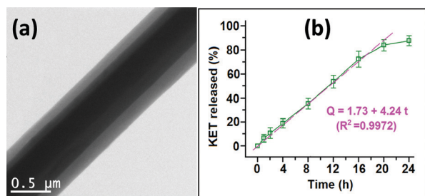
Fig. 5 The triaxial fibres prepared by Yu et al. (a) Transmission electron microscopy image, and (b) the resultant zero-order drug release profile. Adapted with permission from ref. 48 (Yu et al. , 2015). Copyright 2015 American Chemical Society.
