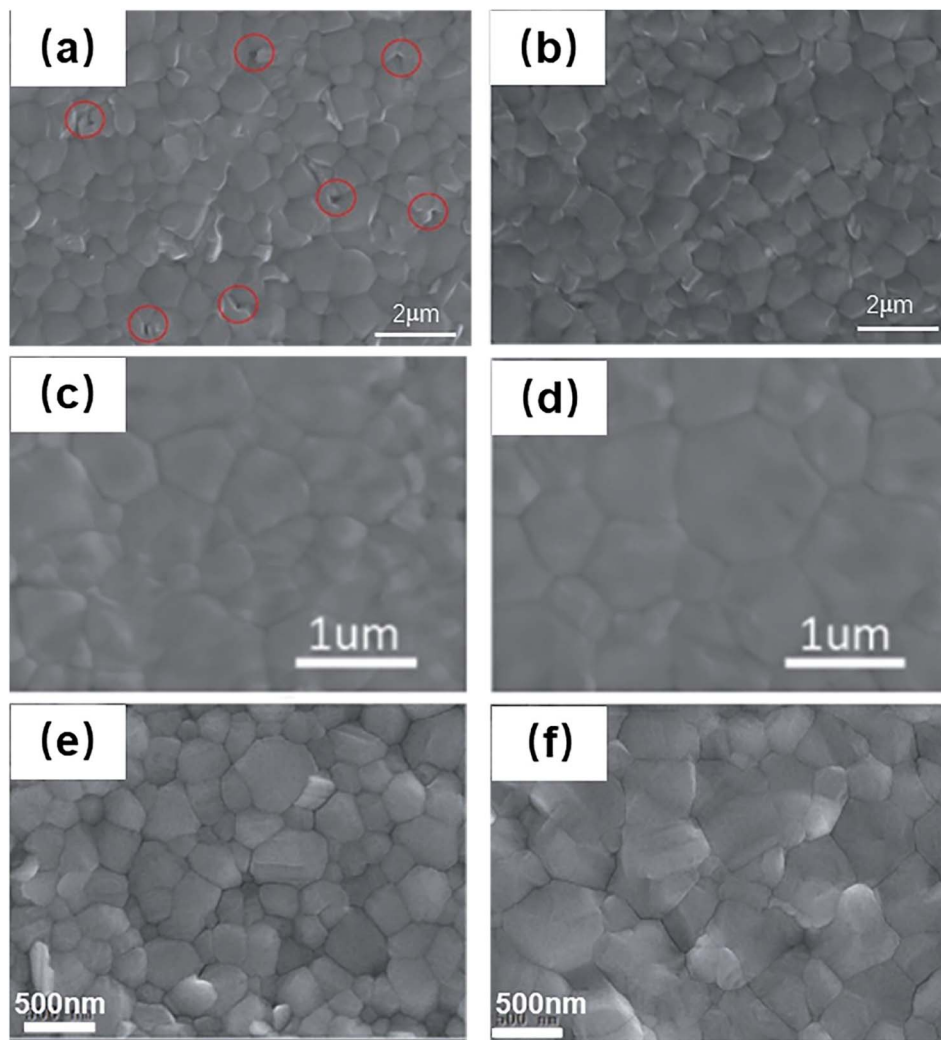
Fig. 9 Top-view SEM images of perovskite films deposited on \text{SnO}_2 and \text{SnO}_2 /metal oxide ETLs. (a) \text{SnO}_2 and (b) \text{In}_2\text{O}_3/\text{SnO}_2 . Reproduced with permission. 245 Copyright 2020, Wiley-VCH. (c) \text{SnO}_2 ; (d) \text{WO}_x/\text{SnO}_2 . Reproduced with permission. 246 Copyright 2019, Elsevier B.V. (e) P- \text{SnO}_2 ; (f) B- \text{SnO}_2 . Reproduced with permission. 247 Copyright 2021, Wiley-VCH.
