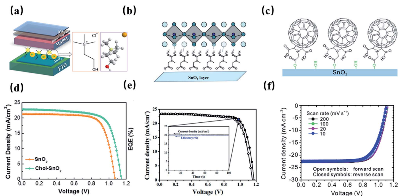
Fig. 13 Schematic illustration of the formation of various self-assembled monolayers adhering to \text{SnO}_2 layers and J - V curve of devices with different SAM treatments. (a and d) Choline chloride treatment. Reproduced with permission. 284 Copyright 2020, ACS Publishing Group. (b and e) 2-[Carbamimidoyl(methyl)amino]acetic acid treatment. Reproduced with permission. 285 Copyright 2015, Royal Society of Chemistry. (c and f) \text{C}_{60} -pyrrolidine tris-acid treatment. Reproduced with permission. 287 Copyright 2020, Nature Publishing Group.
