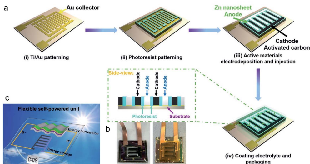
Fig. 19 (a) Fabrication process of ZnSC. (b) Images of ZnSC. Reproduced with permission. 89 Copyright 2019, Wiley-VCH (c) Diagram of the integrated flexible self-powered ZIHC combining ZnSC and miniaturized solar cells. Reproduced with permission. 169 Copyright 2020, Springer Nature.
