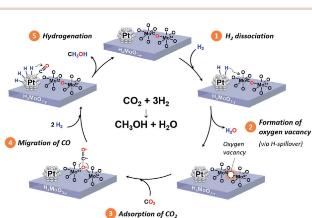
Scheme 2 Proposed reaction mechanism of CO 2 hydrogenation to produce methanol over the Pt/H x MoO 3-y catalyst.
