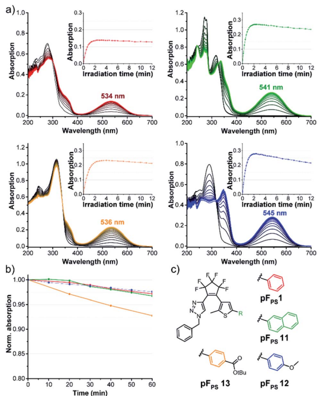
Fig. 5 Photochromic properties of various thieryl substitutions: (a) time-dependent changes of the absorption spectra of 60 \mu\text{M} solutions of pF PS 1, 11–13 upon UV light irradiation (310 nm, LED) in chloroform towards the (pseudo)-photostationary state; insets show the absorption vs. time trace measured at the VIS absorption maximum during extended UV irradiation to analyse the photostability, (b) thermostability (20 °C) of the CF isomers, (c) structures.
