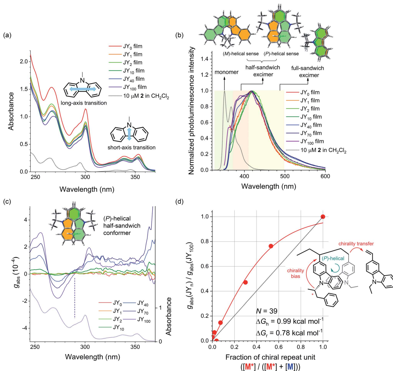
Fig. 3 (a) UV-vis absorption spectra of neat films of the JY n polymers spin-coated onto quartz substrates. The black dotted curve is the UV-vis absorption spectrum of a 10 \mu M solution of 2 (CH 2 Cl 2 ). The insets show the short- and long-axis transitions of carbazole. (b) Fluorescence spectra of neat films of the JY n polymers ( \lambda_{\text{ex}} = 339 nm). The black dotted curve is the fluorescence spectrum of a 10 \mu M solution of 2 (CH 2 Cl 2 ). The colored regions highlight the monomeric emission of carbazole (green) and the carbazole excimer emissions of a half-sandwich conformer (beige) and a full-sandwich conformer (yellow). The structures at the top depict the two half-sandwich conformers and the full-sandwich conformer. (c) Plots of the Kuhn dissymmetry factor ( g_{\text{abs}} ) as a function of wavelength for neat films of the JY n polymers cast onto quartz substrates. See ESI, Fig. S5† for the corresponding ECD spectra. The dotted curve is the UV-vis absorption spectrum of a neat film of the JY 100 polymer. The positive Cotton effect in the long-axis transition reflects the (P)-helical sense of the half-sandwich conformer of carbazoles (see the inset). (d) A plot of the normalized g_{\text{abs}} values ( \lambda = 304 nm) for the JY n polymers (i.e., g_{\text{abs}}(\text{JY}_n)/g_{\text{abs}}(\text{JY}_{100}) ) as a function of the chiral repeat unit fraction in the polymers (i.e., [\text{M}^*]/([\text{M}^*] + [\text{M}]) ). The red curve is the nonlinear least-squares fit of the data to eqn (1). The inset shows the chirality transfer from the chiral monomer to the achiral monomer during the polymerization (see the inset).
