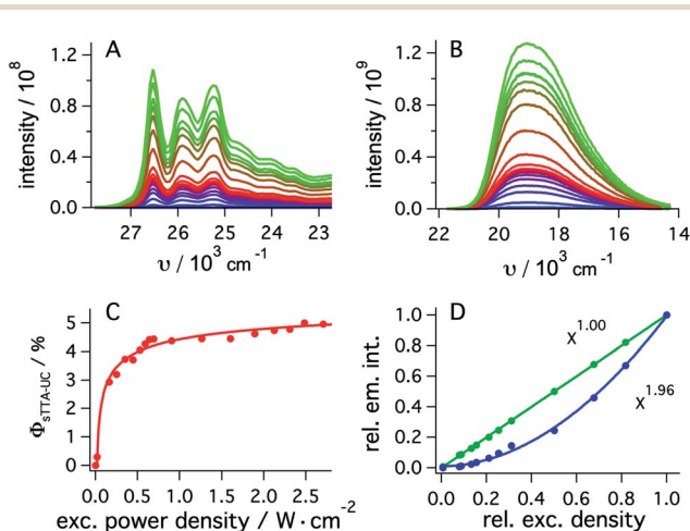
Fig. 4 (A) Upconverted ^t\text{BuPy} fluorescence sensitized by \text{fac}[\text{Ir}(\text{ppy})_3] (30 \mu\text{M} ) in de-aerated DMF at 20 °C. Excitation occurred with a 447 nm cw-laser at various excitation densities in the presence of ^t\text{BuPy} (5 mM). Excitation powers ranged from 2 mW to 338 mW. (B) Emission spectra of \text{fac}[\text{Ir}(\text{ppy})_3] recorded under identical conditions as for (A) but in the absence of ^t\text{BuPy} . (C) Upconversion quantum yield ( \phi_{\text{sTTA-UC}} ) as a function of excitation power density as determined from eqn (1) and the data in (A) and (B), using a luminescence quantum yield ( \phi_{\text{ref}} ) of 0.88 for \text{fac}[\text{Ir}(\text{ppy})_3] . (D) Relative integrated intensities of upconverted ^t\text{BuPy} (1 mM) fluorescence (blue circles) sensitized by \text{fac}[\text{Ir}(\text{ppy})_3] (10 \mu\text{M} ) upon excitation at 450 nm as a function of the relative excitation density. The solid blue line represents the best fit with a power function ( f(x) = a \times x^b + y ) to the experimental data, yielding b = 1.96 as indicated by the inset. The green circles result from an analogous experiment in which \text{fac}[\text{Ir}(\text{ppy})_3] was excited in the absence of ^t\text{BuPy} under otherwise identical conditions, and the prompt luminescence emitted by \text{fac}[\text{Ir}(\text{ppy})_3] was monitored (Section 2.5.2 of the ESI†). In this case, a fit to the same power function (green solid line) yields an exponent of 1.00. Measurements in C occurred with the abovementioned cw-laser source, whilst measurements in D were performed using the excitation beam of the luminescence spectrometer.
