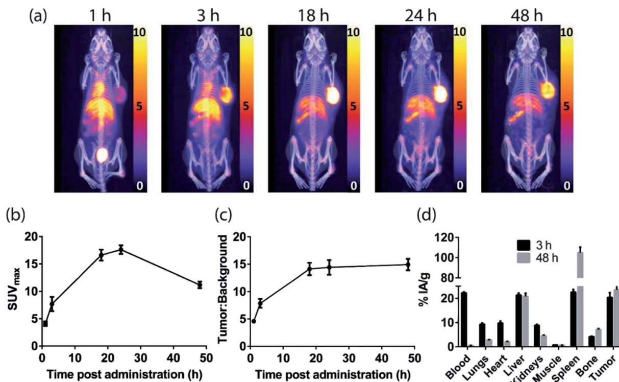
Fig. 6 In vivo results following administration of [^{64}\text{Cu}][\text{CuMeCOSar}]\text{-cetuximab} in A431 xenograft tumor-bearing NSG mice. (a) PET/CT MIP images (scale given in SUV). (b) \text{SUV}_{\text{max}} values (c) tumor : background ratios and (d) ex vivo biodistribution results. All values are given as mean \pm SEM ( n = 3 ).
