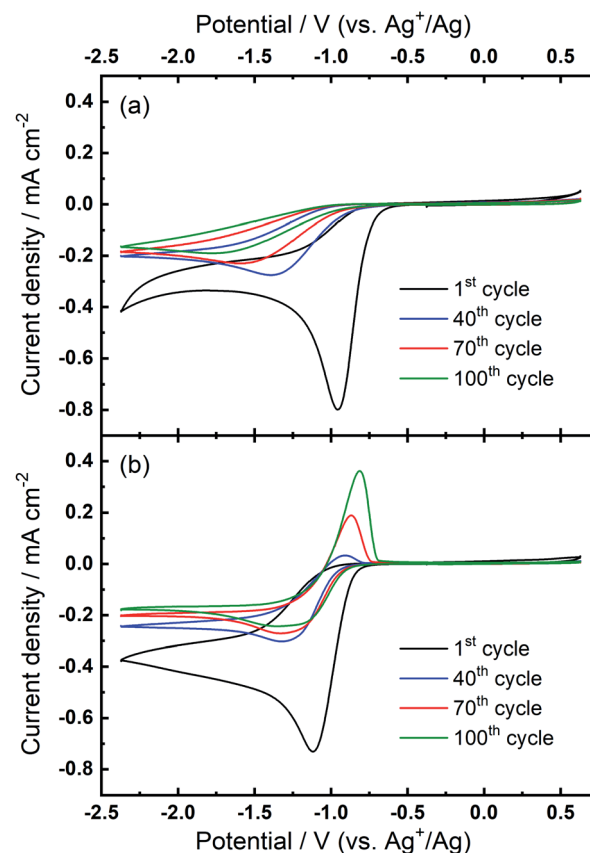
Fig. 2 Cyclic voltammograms of the ORR and OER on Au at 100 \text{ mV s}^{-1} in \text{O}_2 -saturated (a) 0.1 M \text{TBAClO}_4/0.1 M \text{Ca}(\text{ClO}_4)_2/\text{DMSO} and (b) 0.1 M \text{TBAClO}_4/0.01 M \text{Ca}(\text{ClO}_4)_2/\text{DMSO} .
