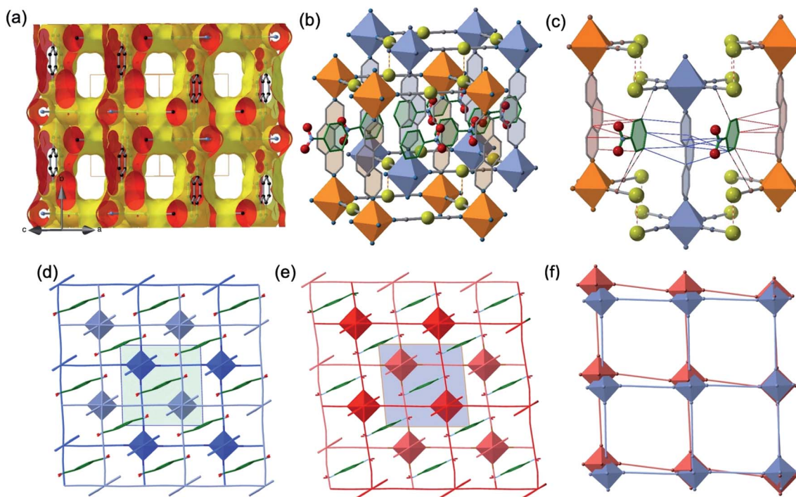
Fig. 4 (Top) View of a fragment of the interpenetrated pcu frameworks illustrating: (a) the solvent-excluded surface showing void channels running along a + c direction; (b) the 1\text{-PhNO}_2 molecules located in the channels (the shown \text{PhNO}_2 molecule represents the average of two slightly disordered positions); and (c) \text{C}_{(3,8\text{-phen})}\cdots\text{C}_{(\text{PhNO}_2)} (red, blue thin bonds) and \text{C}_{(\text{Au}(\text{CN})_2)}\cdots\text{C}_{(\text{PhNO}_2)} (black-red thin bonds) intermolecular interactions shorter than the sum of van der Waals radii at 228 K. Red-white thin bonds correspond to the Au \cdots Au interactions between the two interpenetrated frameworks. (Bottom) View down to [010] direction of the interpenetrated frameworks marked in light- and dark-blue LS state (d), light- and dark-red (HS state) (e) including the \text{PhNO}_2 molecule located in the channels (the inner green/blue squares correspond to the unit cell); (f) superposition of one of the two frameworks illustrating the distortion of the structure when moving from the LS state (blue) to the HS state (orange).
