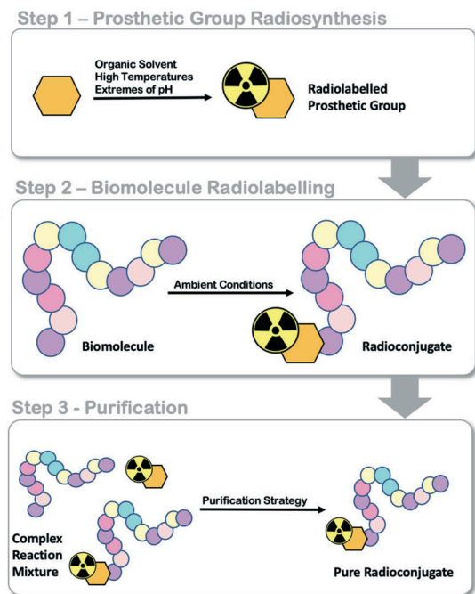
Fig. 1 Schematic representation of fluorine-18 prosthetic group (PG) strategies for radiolabelling peptides and proteins.
