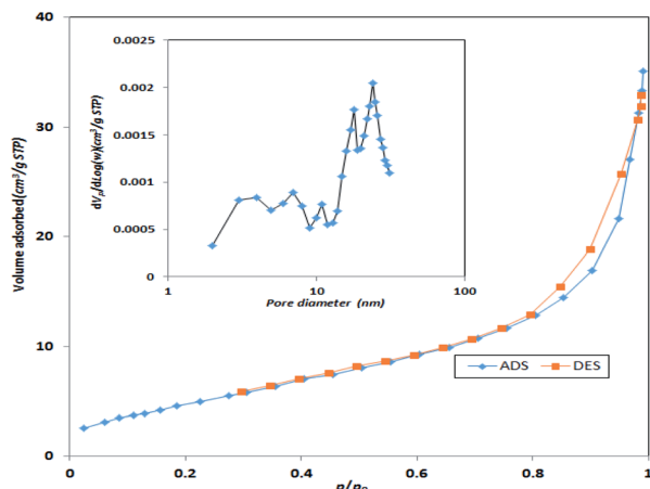
Fig. 5 \text{N}_2 adsorption-desorption isotherms of MgO catalyst.
