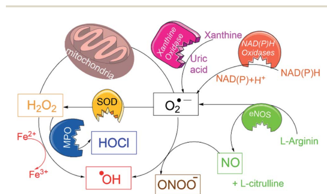
Fig. 1 Schematic overview for generation of a variety of ROS/RNS species in biological conditions and their interconversions.
