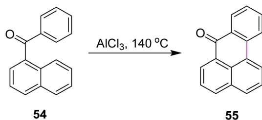
Scheme 23 \text{AlCl}_3 -mediated Scholl reaction of benzoylnaphthalene. 52
