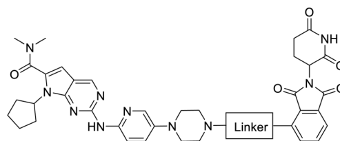
Ribociclib - based degrader
