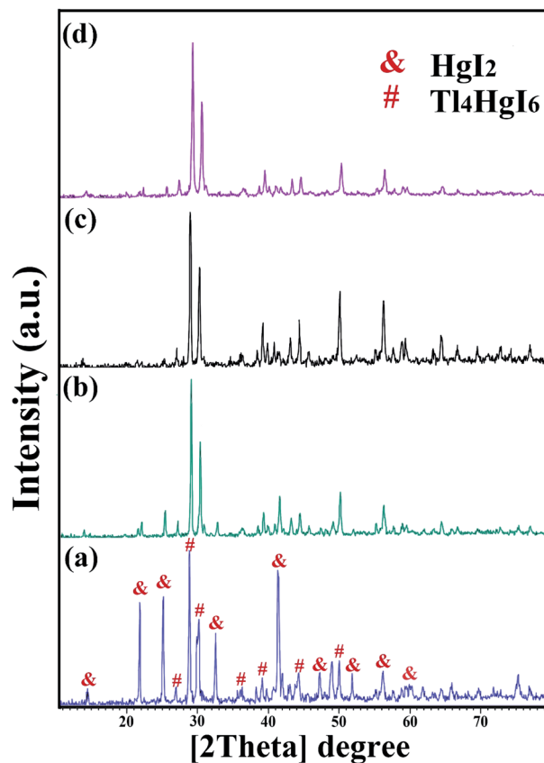
Fig. 1 XRD patterns obtained from Tl 4 Hgl 6 /Hgl 2 nanocomposite in different ratios of Tl to Hgl 2 precursors; (a) 1 : 1, (b) 2 : 1, (c) 3 : 1, and (d) 1 : 2.
