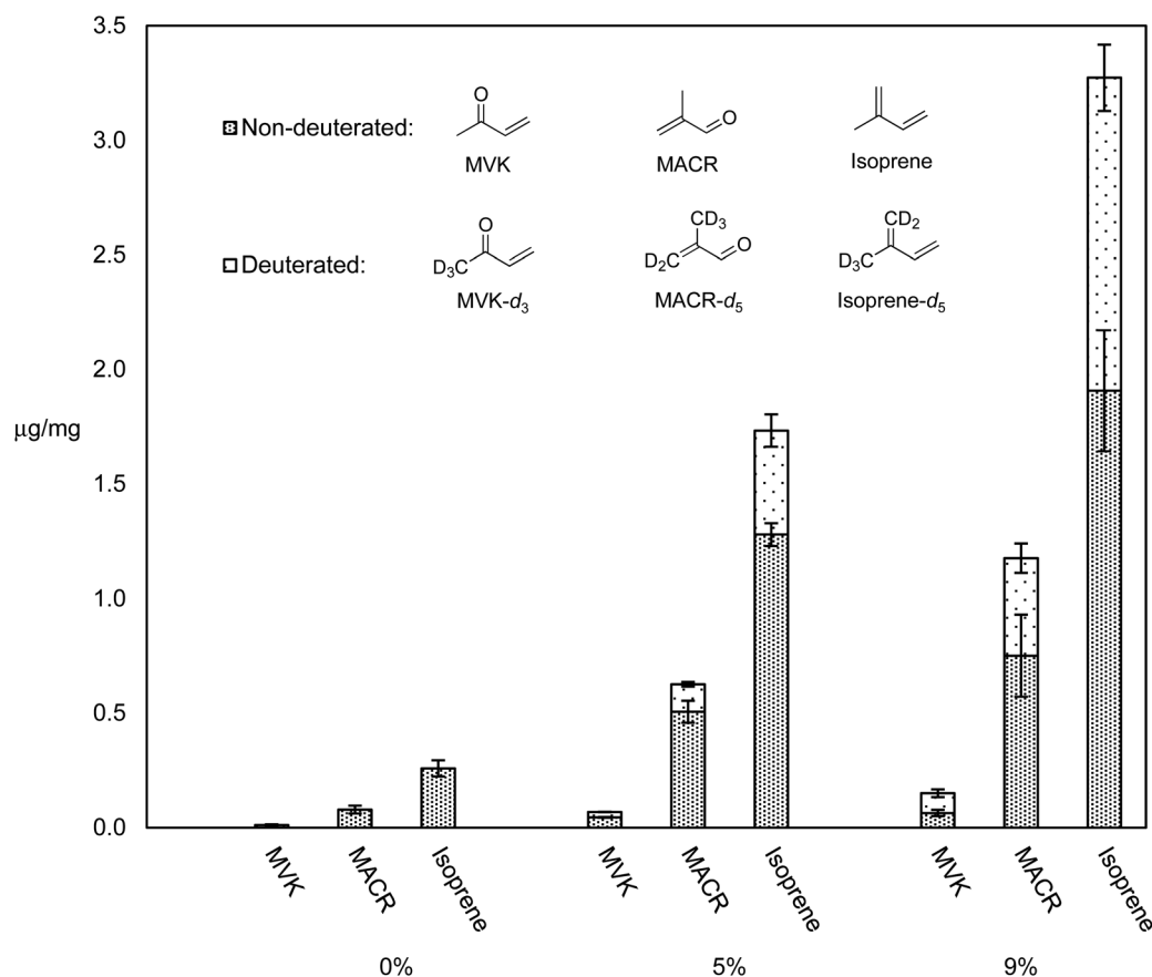
Fig. 4 Comparative levels of major degradation products and their deuterated isotopologues encountered in the aerosol GP from dabbing pure THC (0% β-myrcene- d 6 ), THC with 5% β-myrcene- d 6 , and THC with 9% β-myrcene- d 6 . Error bars are SEM.
