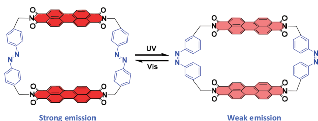
Fig. 1 Schematic illustration of PBI cyclophane supramolecular elements. (a) Representative PBI cyclophane supramolecular elements with rigid linkers. (b) PBI cyclophane supramolecular element with photoresponsive linkers, which showed reversible structural and fluorescence switching under alternate UV and visible light irradiation. Notes: The bay-position substituents of the PBIs are omitted for clarity. For details of the PBI cyclophane structures illustrated in (a), the original literature reports 21–25 should be consulted.
