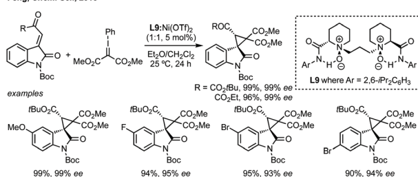
Scheme 5 Ni-Catalysed enantioselective cyclopropanation with phenyliodonium derived ylides.
