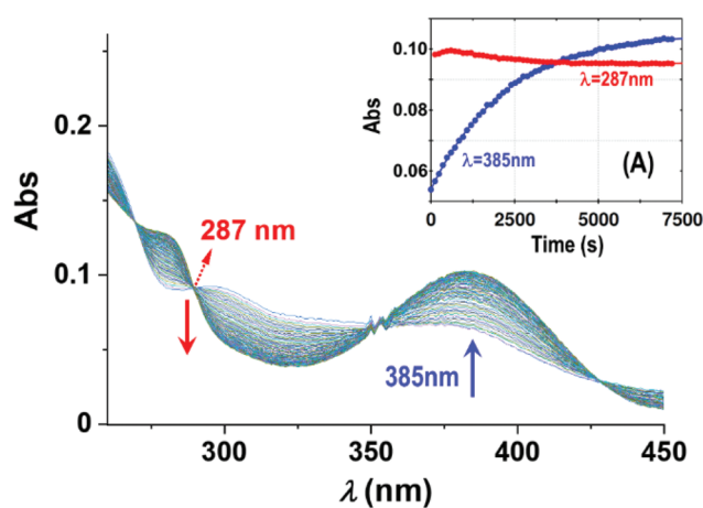
Fig. 6 Absorbance changes of 1-OH 2 (16 \mu\text{M} ) around the isosbestic point (287 nm) with time in the presence of PPI (10 equiv.; 0.16 mM) at pH 7.35 ([Tris buffer] = 10 mM) and 12 °C illustrating the presence of earlier reactions. Inset (A): L.S. fits of Abs vs. time at 287 nm (red) and 385 nm (blue), respectively, showing the small absorbance changes of the first reactions (induction period) and underlining the small absorbance changes therewith, not influencing the individual fits and kinetic data as illustrated in the k_{\text{obs}} vs. [\text{PPI}]_{\text{tot}} graph in Fig. 3 and 5.
