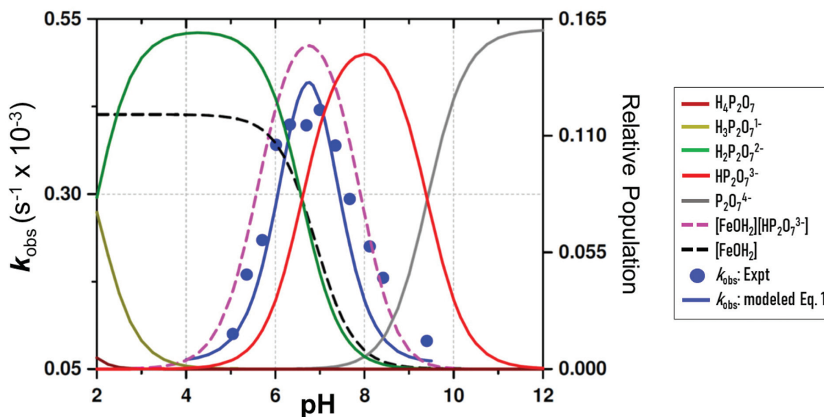
Fig. 4 pH dependence of the observed pseudo first-order rate constant ( k_{\text{obs}} ) (blue points) for the reaction between 1-OH 2 (16 \mu\text{M} ) and PPI (10 equiv.; 0.16 mM) at 25 °C. The line (blue curve) shows a modeled fit from all data at 25 °C, including those obtained from the fluorescence traces at 28 °C to the overall total rate law expression, eqn (1). This was obtained using k_{\text{PPI}} = 3.1 \times 10^{-3} \text{ s}^{-1} ; and K_{\text{eq}} = 2700 \text{ M}^{-1} , as well as a slow reaction concurrent to k_{\text{PPI}} , as intercept, k_{22} = 6.0 \times 10^{-5} \text{ s}^{-1} , to model the best visual fit [restrained to within the large relative standard deviations as expected: (i) due to the complexity of the system and model utilised, and (ii) having two dependent variables simultaneously] for the parameters k_{\text{PPI}} and K_{\text{eq}} . Also shown are relative speciation curves of PPI vs. pH, correlated to the pH dependency of k_{\text{obs}} , as well as the pH speciation of 1-OH 2 (black). These are all compared to the product of the populations of 1-OH 2 and \text{HP}_2\text{O}_7^{3-} (pink).
