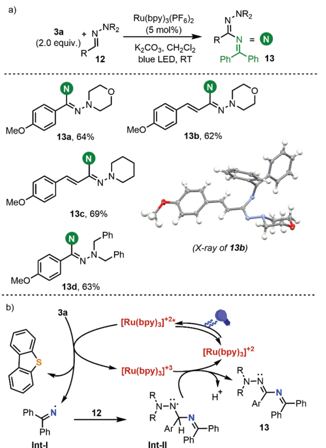
Scheme 6 (a) Synthesis of hydrazonamides 13 and (b) plausible reaction mechanism.
