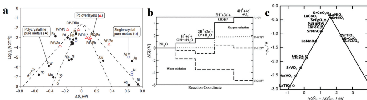
Fig. 2 (a) A volcano plot of experimentally measured exchange current density as a function of the calculated \Delta G_{\text{H}^*} . 27 (b) The free energy diagram for OER steps (from left to right) at different applied potentials ( U ). Due to the scaling relation between the free energy of the intermediates ( \text{OH}^* , \text{O}^* , \text{OOH}^* ), they are correlated and thus moved in a concerted manner. At U = 2.55 V, all the OER steps are exothermic (downhill from left to right). 34 (c) Activity trends of the perovskite OER electrocatalysts. The negative theoretical overpotential was plotted against the difference of standard free energy of the ( \Delta G_{\text{O}^*} - \Delta G_{\text{OH}^*} ) step. 22
