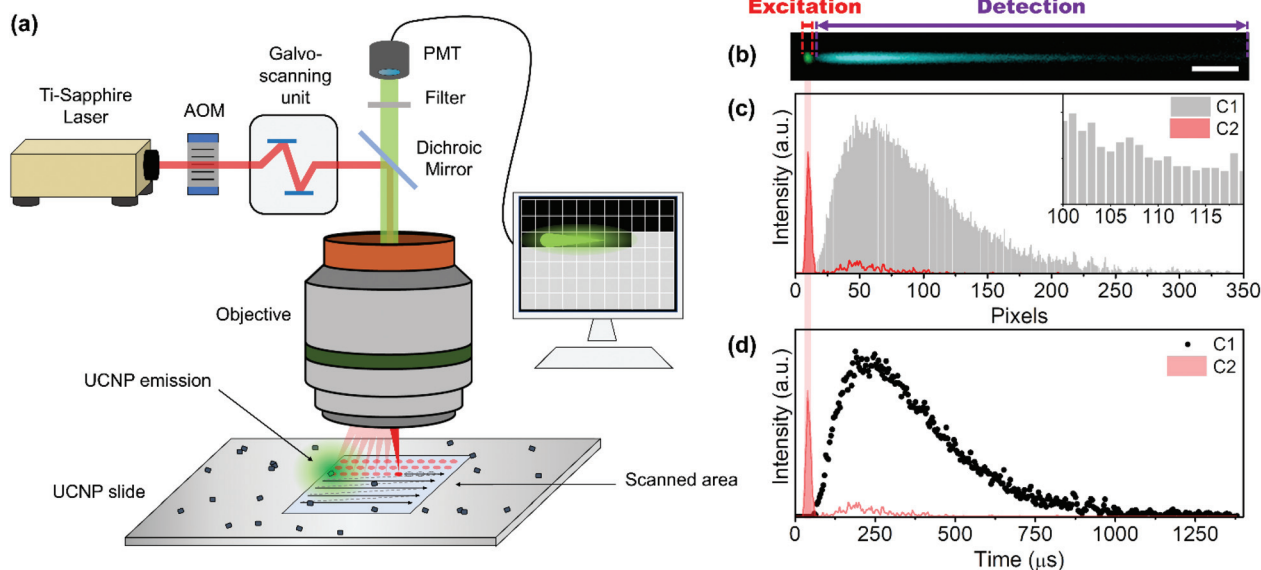
Fig. 2 Scheme and visual representation of the time-resolved principle of NIR-LSM. (a) NIR-LSM scheme. (b) Composite image of image of the UCNP emission (blue, detection channel 1) and Rh110 two-photon excitation emission (green, detection channel 2) at 975 nm excitation and 4 \mu s per pixel dwell time of the same agglomerate of UC Tm @Rh110 UCNH ( F_d = 10.4 J cm -2 ). Scale bar 20 \mu m. (c) Intensity profiles and (d) kinetic profiles obtained from image (a).
