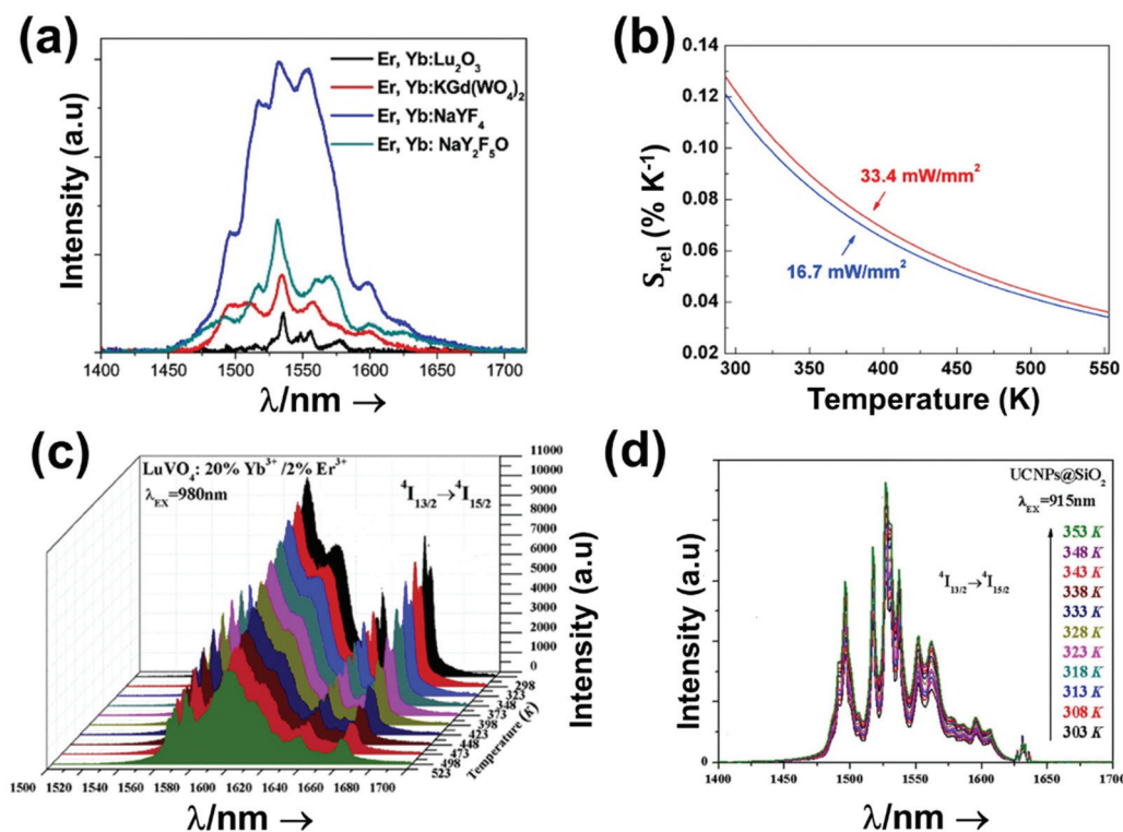
Fig. 42 (a) Intensity of the \text{Er}^{3+} 1550 \text{ nm} emission in different hosts after excitation at 980 \text{ nm} . Reprinted with permission from ref. 265. Copyright Elsevier. (b) Effect of the excitation power density at 980 \text{ nm} in S_{\text{rel}} of \text{Er}^{3+}, \text{Yb}^{3+}:\text{BaMoO}_4 nanoparticles. Reprinted with permission from ref. 269. Copyright 2018, Elsevier. (c) Temperature dependence of the intensity of the \text{Er}^{3+} 1550 \text{ nm} emission in \text{Er}^{3+}, \text{Yb}^{3+}:\text{LuVO}_4 nanoparticles, excited at 980 \text{ nm} . Reprinted with permission from ref. 267. Copyright 2018, Elsevier. (d) Temperature dependence of the intensity of the \text{Er}^{3+} 1550 \text{ nm} emission in \text{LuVO}_4@\text{SiO}_2 core-shell nanoparticles, excited at 915 \text{ nm} . Reprinted with permission from ref. 268. Copyright 2019, American Chemical Society.
