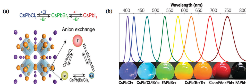
Fig. 5 (a) Schematic of the halide anion-exchange process. Reproduced with permission from ref. 38 at https://pubs.acs.org/doi/abs/10.1021/acscnanolett.5b02404 ; further permissions are directed to the ACS. (b) Photoluminescence spectra and the corresponding photographs (under varied daylight and UV excitation) of colloid composition-tuned APbX 3 NCs. From ref. 92, reprinted with permission from AAAS.
