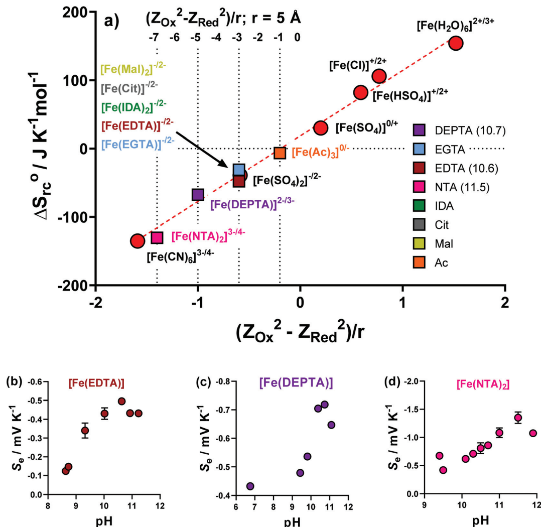
Fig. 7 Showing (a) a plot of \Delta S_{rc} vs. (Z_{\text{Ox}}^2 - Z_{\text{Red}}^2)/r for previously reported aqueous Fe(II)/Fe(III) redox systems (red circles) and all Fe(ligand) solutions investigated here (coloured squares). The dotted lines indicate the (Z_{\text{Ox}}^2 - Z_{\text{Red}}^2) values of 0/–1, –1/–2, –2/–3 and –3/–4 redox couples (using r = 5 \text{ \AA} ). From these the likely ionic charge changes in the redox couples have been put next to the complex, e.g. [\text{Fe}(\text{NTA})_2]^{3-/4-} . The values for Fe(EDTA), Fe(DEPTA) and Fe(NTA) were the pH optimised values (pH values specified in brackets in the legend); (b), (c) and (d) plot the observed trends in S_e vs. pH for these three, respectively, using an applied \Delta T = 20 \text{ K} . pH modification was achieved by the direct addition of solid \text{K}_2\text{CO}_3 to the semi-optimised systems.
