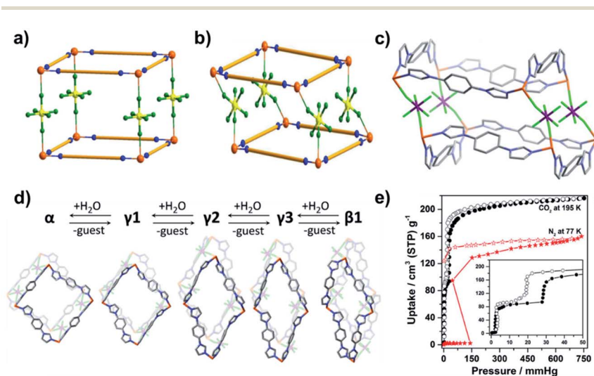
Fig. 12 Schematic diagrams of (a) traditional SIFSIX- n - M networks with trans -bridging SIFSIX pillars and (b) SIFSIX-23-Cu with cis -bridging SIFSIX pillars; (c) coordination mode and geometry in SIFSIX-23-Cu; (d) reversible structural transformations in SIFSIX-23-Cu; (e) \text{N}_2 (77 K) and \text{CO}_2 (195 K) sorption isotherms of SIFSIX-23-Cu. Reproduced from ref. 151 with permission; copyright: 2020, American Chemical Society.
