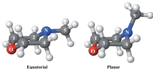
Fig. 1 The equatorial and planar structures of NMM.
