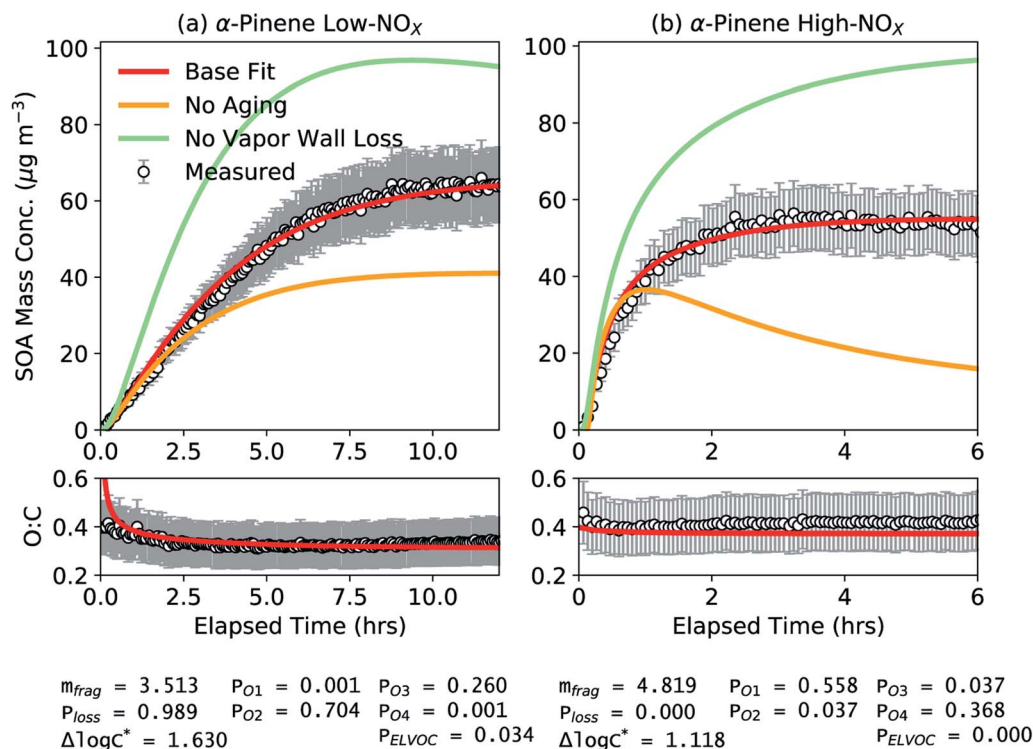
Fig. 1 SimpleSOM predictions of SOA mass concentration and SOA O : C ratio compared to measurements for (a) low and (b) high NO x photooxidation experiments performed on α-pinene. 81 Model predictions based on fits to the SOA mass concentration and O : C are shown in solid red while those for simulations using the base fit parameters but with no multigenerational aging or no vapor wall losses are shown in solid mint and orange, respectively. The fit parameters for the respective NO x conditions are listed at the bottom of the figure.
