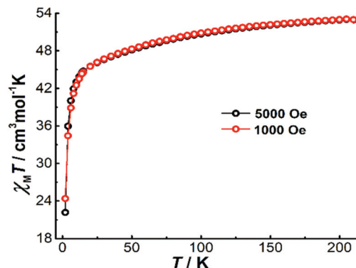
Fig. 3 Temperature dependence of the product \chi_M T for \text{Dy}_4 at indicated fields between 2 and 210 K.
