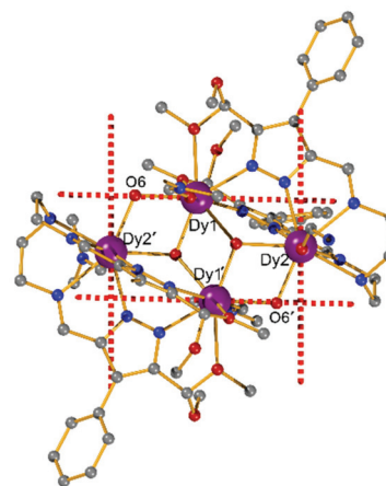
Fig. 4 Orientations of the main magnetic axes of the local magnetizations in the ground state of \text{Dy}_4 .
