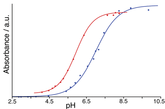
Fig. 7 pH titrations showing the change in absorbance arising from deprotonation of BCP in the absence (blue), and presence (red), of excess H W in water. Derived \text{pK}_\text{a} values are in the main text; the stabilisation of the deprotonated form of BCP by ca. 1 \text{pK}_\text{a} unit in the presence of H W is clear. In both cases small circles represent measured data and the solid lines represent the best calculated fit to a pH curve.
