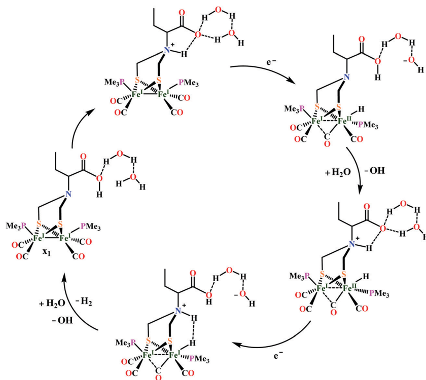
Scheme 27 Proposed mechanism for the electrocatalytic proton reduction mediated by [\text{Fe}_2(\text{CO})_4(\text{PMe}_3)_2\{\mu\text{-SCH}_2\}_2\text{NCH}(\text{CH}_2\text{CH}_3)\text{COOH}] (Fig. 28x 1 ) in aqueous medium, explaining the role of the -\text{COOH} group as a proton transfer relay. 461
