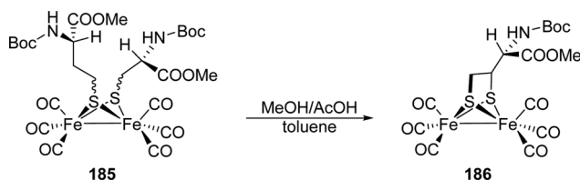
Fig. 56 Intramolecular cyclization of 185 resulting in 186 .
