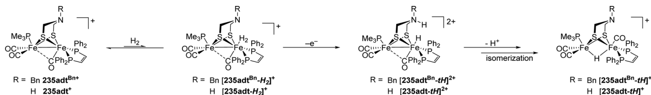
Fig. 84 Hydrogen oxidation by complexes \mathbf{235adt}^{\text{R}+} .
