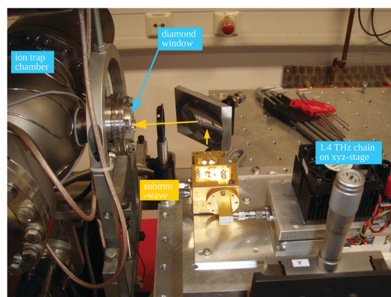
Fig. 6 (Upper scheme) Experimental setup for rotational action spectroscopy of \text{H}_2\text{D}^+ and \text{D}_2\text{H}^+ , consisting of the ion trapping machine and the THz source. (bottom photo) The unit consisting of THz source and ellipsoidal mirror is placed on a common support (simple bread board), which has been moved between the trapping machine and a test setup on a nearby optical bench for adjustment and power calibration. The scheme is reprinted from ref. 45 with permission of APS.
