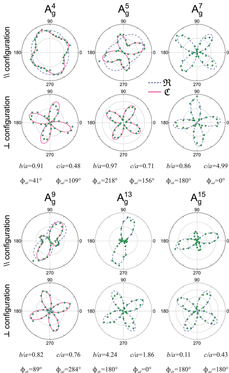
Fig. 8 Typical Raman polar plots of a monolayer triclinic \text{ReSe}_2 . Angular dependence of the intensities of 6 A_g modes in the parallel (||) and crossed (⊥) configurations for an exfoliated monolayer \text{ReSe}_2 collected using an excitation energy of 2.33 eV. The corresponding tensor element ratios and phase differences extracted from the fitting process are also shown. Adapted with permission from ref. 19.
