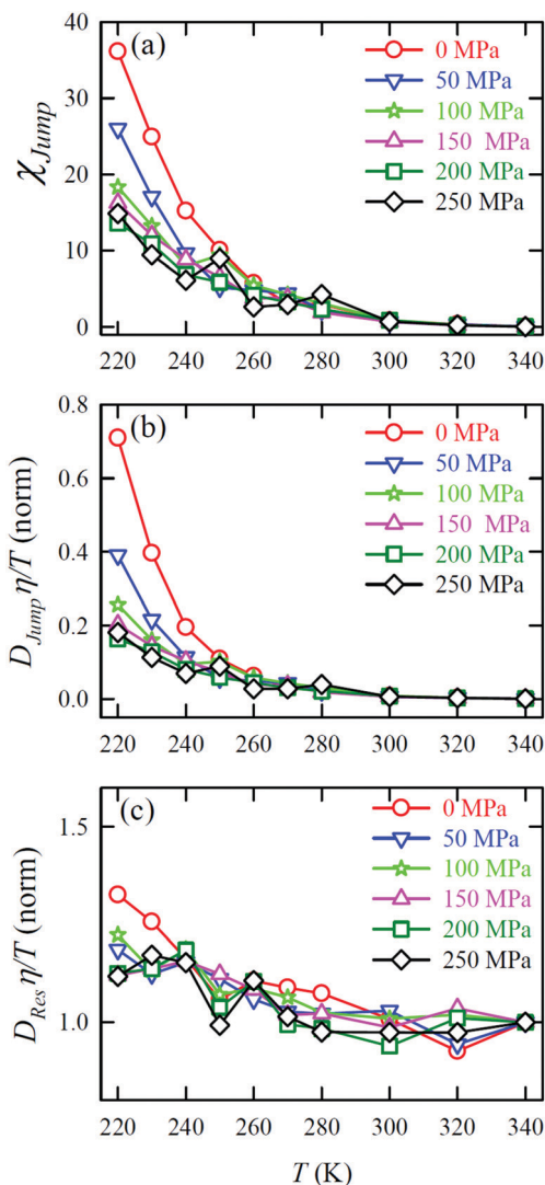
Fig. 11 (a) Temperature-dependent percentage contribution \chi_{\text{Jump}} for different pressures. (b) Normalized D_{\text{Jump}}\eta/T , and (c) Normalized D_{\text{Res}}\eta/T as functions of temperature for all pressures. The normalization is done at T = 340 K. Reprinted with permission from ref. 65. Copyright (2019) American Chemical Society.
