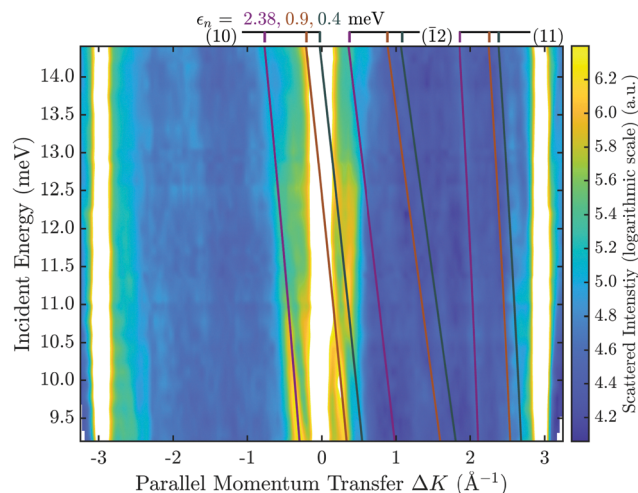
Fig. 6 Contour plot of the scattered He intensity in dependence of momentum transfer and incident energy along the \Gamma\bar{K} azimuth, for the \text{Sb}_2\text{Te}_3(111) sample at 113 K. The solid lines are the positions of the SAR features according to the free atom model with the different colours denoting the bound state energies \epsilon_{1,2,3} . The Miller indices of the interacting \mathbf{G} -vectors are given in brackets.
