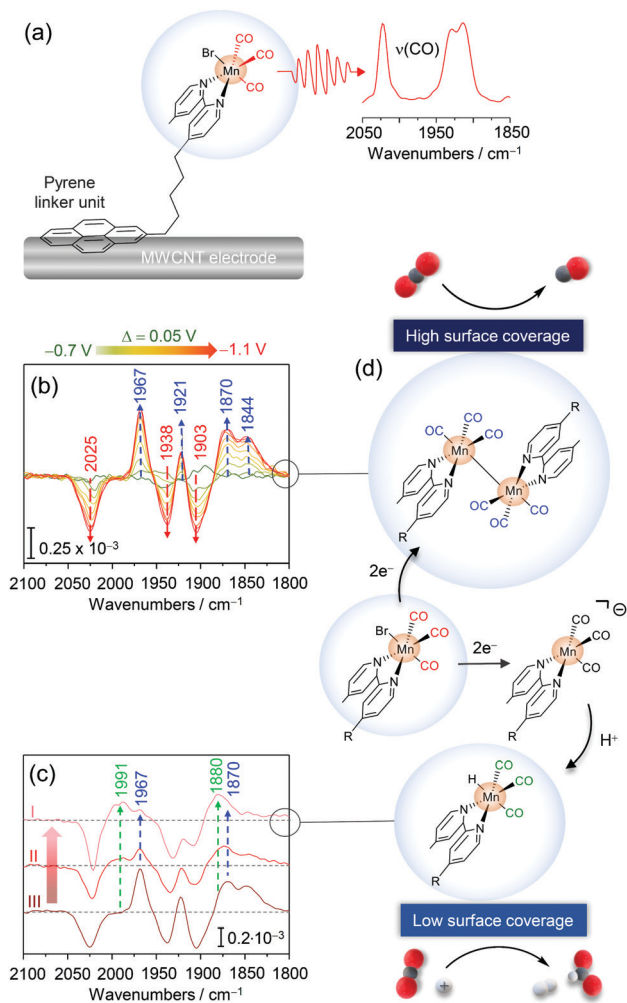
Fig. 6 (a) Pyrene modified Mn fac -tricarbonyl complex immobilised on a multi-walled carbon nanotube (MWCNT) electrode. (b) Potential dependent EC-IR difference spectra revealing the formation of the Mn–Mn dimer species (blue arrows) upon reduction of the parent Mn Pyr species (red arrows). (c) EC-IR difference spectra with decreasing surface coverages of Mn Pyr (from III to I) revealing the formation of a Mn hydride species (green arrows). (d) Scheme for surface coverage dependent redox chemistry and catalytic CO 2 RR selectivity of immobilised Mn Pyr . Graphs and schemes redrawn from ref. 68.
