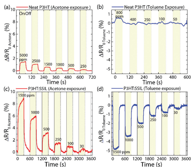
Fig. 4 Percentage change in electronic resistance under acetone and toluene exposure at varying concentrations (ppm) for (a) and (b) neat P3HT and (c) and (d) the P3HT: SSIL 1 : 5 blend under an applied voltage V_D = 2 V.
