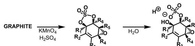
Scheme 1 Organosulfates present in GO prepared via the Hummers' method have been shown to be susceptible to hydrolysis, leading to the formation of acidic sulfate species in the final product. Reproduced from ref. 6 with permission from the Royal Society of Chemistry.
