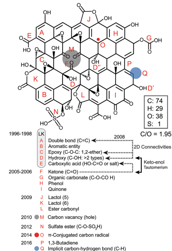
Fig. 2 Structural account of a nanosheet of graphene oxide (GONs) with a C/O ratio of ~2.
