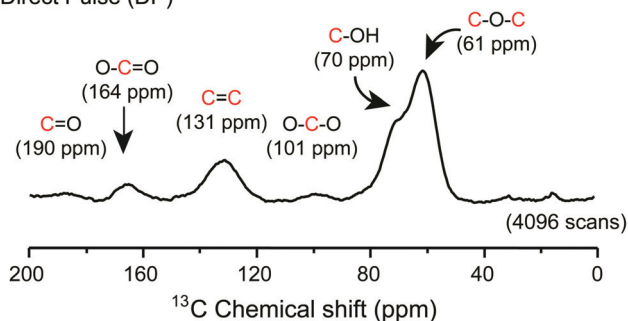
Fig. 4 ^1\text{H} - ^{13}\text{C} cross-polarization (CP) and direct pulse (DP) ^{13}\text{C} - ^1\text{H} decoupled SS-NMR spectra of graphene oxide. ^{13}\text{C} -SS-NMR/MAS spectra were recorded at frequencies of 150.874 MHz for ^{13}\text{C} and 599.84 MHz for ^1\text{H} using a 4 mm magic-angle spinning (MAS) double resonance probe and a zirconium oxide rotor for NMR analysis. Magic angle spinning was performed at a spinning frequency of 12.5 kHz. Typically, 80 mg of dry GO material was used in the sample and 60 000 and 4096 scans were recorded respectively for CP and DP to achieve the desired spectral resolution. All spectra were collected at room temperature (23 °C). Data were analyzed using the Mestrenova ® software (Mestrelab research). Exponential line broadening functions of 50 Hz were applied to the MAS spectra and chemical shifts were referenced relatively to adamantane (38.25 ppm). Cross-polarization- ^{13}\text{C} -SS-NMR/MAS experiments were carried out using a spectral width of 75 kHz, radio-frequency fields of 75 kHz for ^{13}\text{C} and 87.5 kHz for ^1\text{H} with a 30% ramp, a 500 \mu\text{s} contact time, a 3 s recycle delay and an acquisition time of 20 ms. Direct pulse- ^{13}\text{C} -SS-NMR/MAS spectra were recorded using a broadband proton decoupling at a RF field of 87.5 kHz during acquisition, with a spectral width of 75 kHz, a 90° pulse length of 3.3 \mu\text{s} , a 20 s recycle delay and an acquisition time of 20 ms. Reproduced from ref. 21 with permission from Wiley-VCH.
