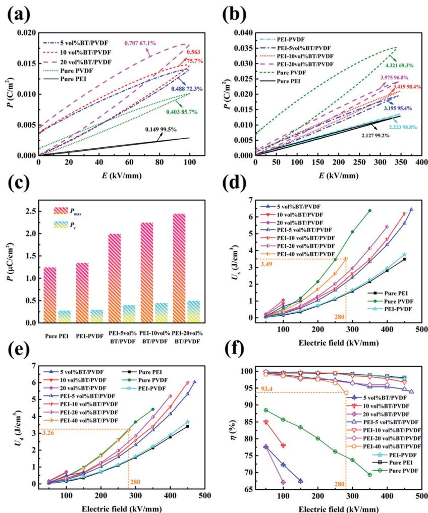
Fig. 5 P - E loops of (a) single layer composites and (b) bilayer composites with different \text{BaTiO}_3 loadings. (c) The maximum displacement P_{\text{max}} and remnant displacement P_r of the pure PEI and bilayer composites at 350 \text{kV mm}^{-1} . (d) The storage energy densities, (e) discharge energy densities and (f) discharge efficiencies of the single layer and bilayer composites under varied external electric fields.
