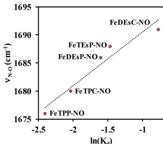
Fig. 7 Correlation between experimentally measured N–O stretching frequency and NO dissociation constant.
