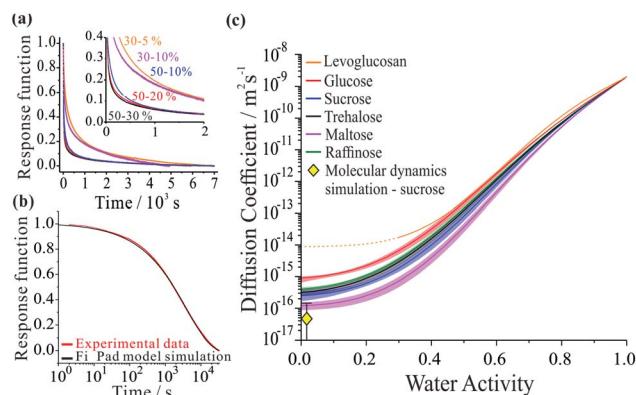
Fig. 1 Examples of each step in the workflow required to extract the compositional dependencies the diffusion coefficients from a time-dependence in particle size. The panels show: (a) a collection of response functions for size changes of aqueous-raffinose particles following a step change in RH; (b) a single response function following a change in RH from 30 to 5% RH for a sucrose particle and the best-fit produced by the Fickian diffusion model. (c) The estimated compositional dependencies of the diffusion of water in the six binary aqueous-organic aerosol systems studied. The estimate of the diffusion coefficient for water in sucrose from the MD simulations also presented (yellow diamond).
