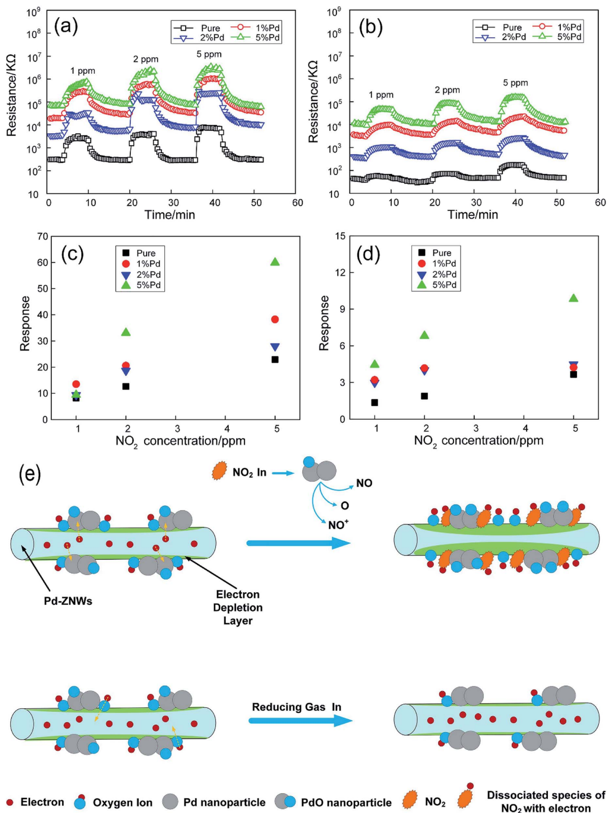
Fig. 3 Dynamic responses of the sensors based on pure ( @150^\circ\text{C} ) and Pd-ZNWs ( @100^\circ\text{C} ) upon exposure to \text{NO}_2 gas with various concentrations at (a) 30% RH and (b) 60% RH. The corresponding sensor responses as a function of \text{NO}_2 concentration at (c) 30% RH and (d) 60% RH. (e) Sensing mechanisms of Pd-ZNWs towards \text{NO}_2 and reducing gas. This figure has been reproduced with permission from ref. 91, Elsevier, Copyright 2019 (License Number: 4923990843354).
