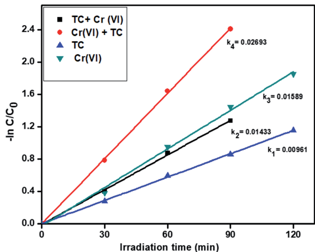
Fig. 8 The kinetics data for the simultaneous removal of TC oxidation and Cr(vi) reduction (120 min of irradiation time, 50 mg L -1 of catalyst R, 20 ppm of TC, 20 ppm of Cr(vi), pH = 5 of TC, pH = 4 of Cr(vi)).
