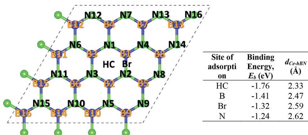
Fig. 1 Different adsorption sites for Ce. The system comprises of a 4 \times 4 \times 1 unit cell of h-BN. Blue (dark) and neon green (light) balls represent boron and nitrogen atoms, respectively. Each atom in a unit cell is identified by a unique index labeled on top of it. The four sites of adsorption: HC (hollow hexagon center), B (on top of any B atom), N (on top of any N atom), and Br (on top of the midpoint of B–N bridge) are also labeled. The corresponding table lists the binding energy ( E_b ) of Ce at the four different sites on h-BN and the perpendicular distance of the Ce adatom from the basal plane of h-BN ( d_{\text{Ce-hBN}} ).
