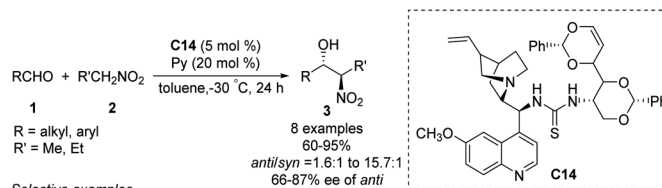
Scheme 36 Cinchona alkaloid catalyst C14 catalyzed Henry reactions.
